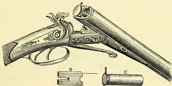
The Original Lefauchaux Breech-loader: 1835.
